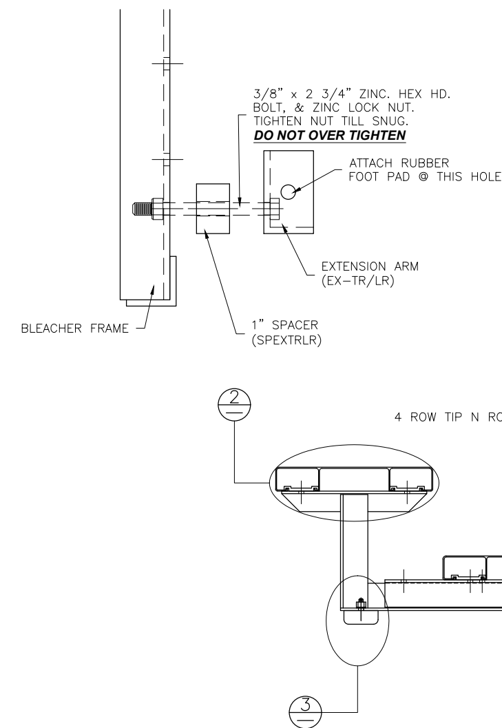
EXTENSION ARM ATTACHMENT DETAIL
